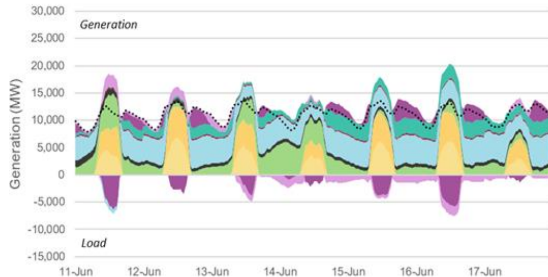
7-day VRE lull in June 2034-35
